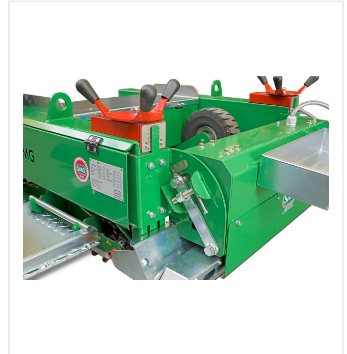
Tilt adjustment of the screed, manual handwheel for adjusting the installation thickness
